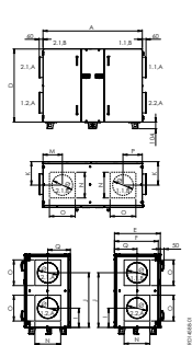
Abmessungen VEX1000CS Monoblock
