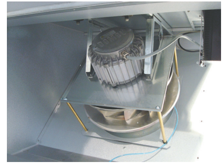
The motor sections are mounted in vibration dampers, which reduces noise in the ducts and eliminates the need to fit flexible connections between the unit and the duct system.
