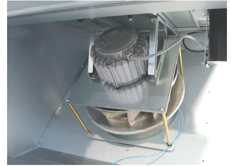
The motor sections are mounted in vibration dampers, which reduces noise in the ducts and eliminates the need to fit flexible connections between the unit and the duct system.
